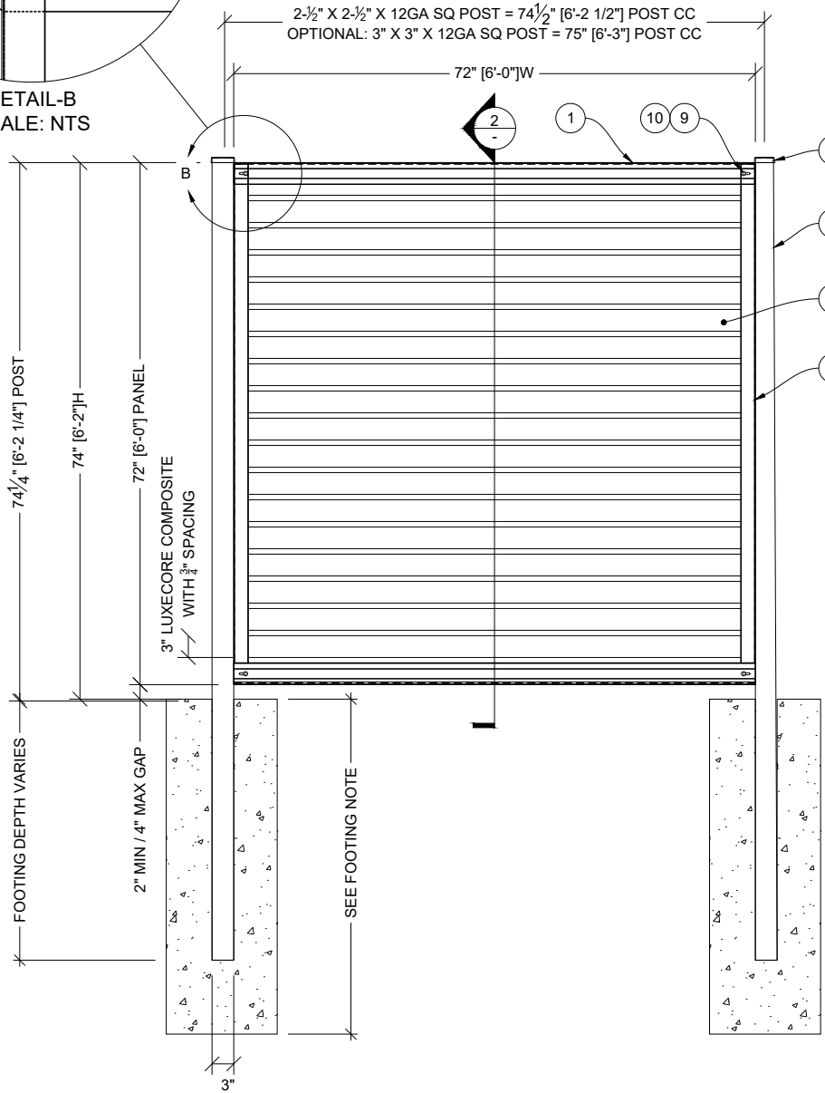
1 FRONT VIEW SCALE: 1/2" = 1'-0"
